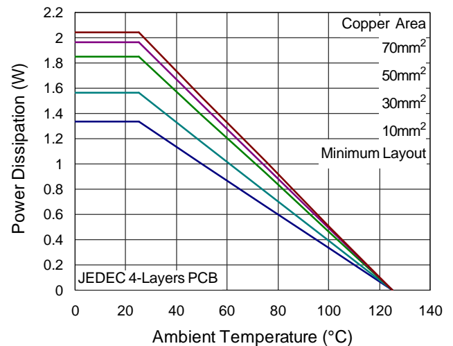
Figure 4. De-rating Curves
