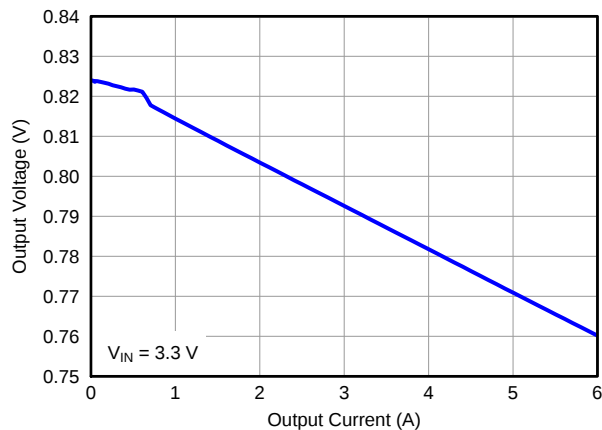
Figure 9. 0.8-V Load Regulation ( V_{IN} = 3.3\text{ V} )
