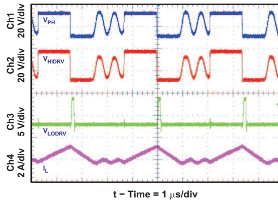
t – Time = 1 μs/div Figure 33.
