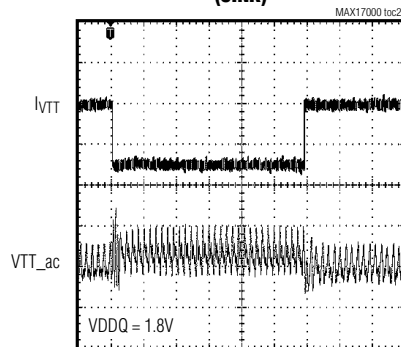
VTT LOAD-TRANSIENT RESPONSE
