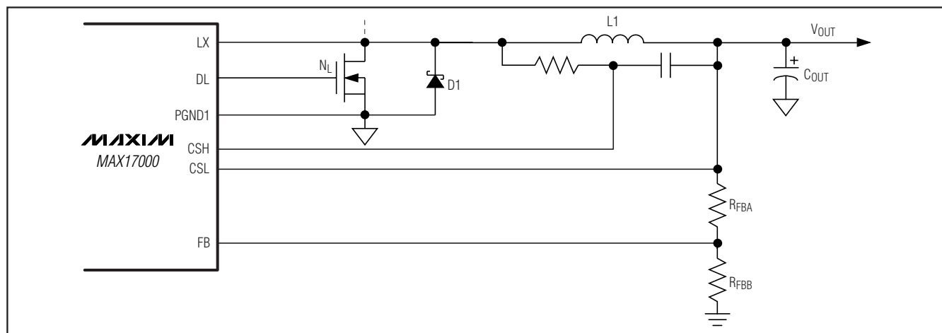
Figure 8. Setting V_{OUT} with a Resistive Voltage-Divider
