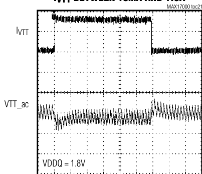
VTT LOAD-TRANSIENT RESPONSE (SOURCE)
