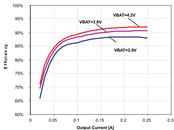
OTG BOOST EFFICIENCY V BUS = 5.5 V
