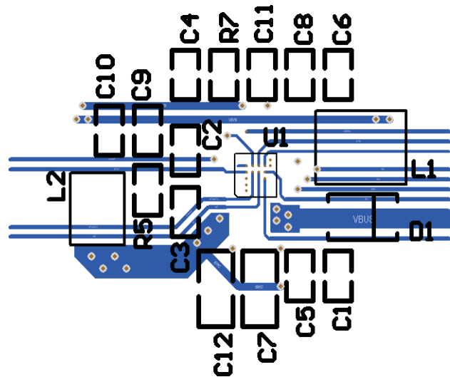
Figure 60. TOP: Top Layer PCB Layout. BOTTOM: Bottom Layer PCB Layout.
