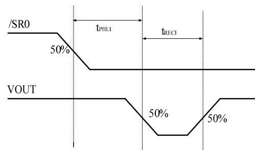
Figure 20. Reset Timing
