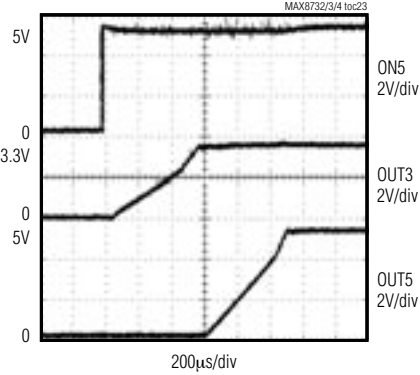
DELAYED START WAVEFORMS (ON5 = REF)
