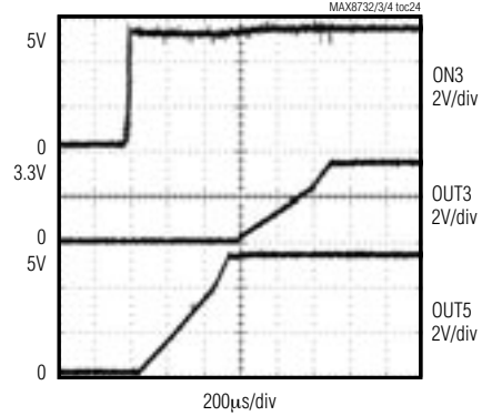
DELAYED START WAVEFORMS (ON3 = REF)
