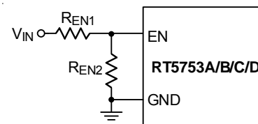
Figure 8. Resistive Divider for Under-Voltage Lockout Threshold Setting
