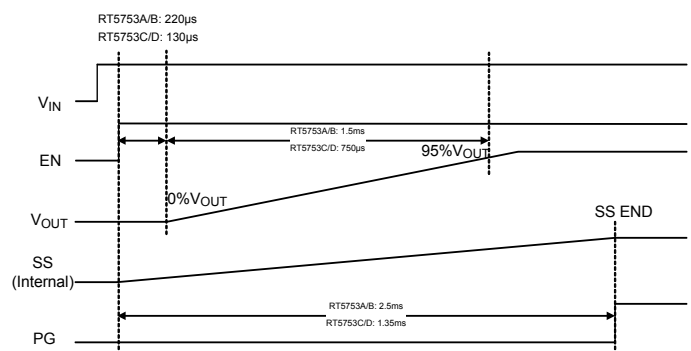
Figure 1. Start-Up Sequence
