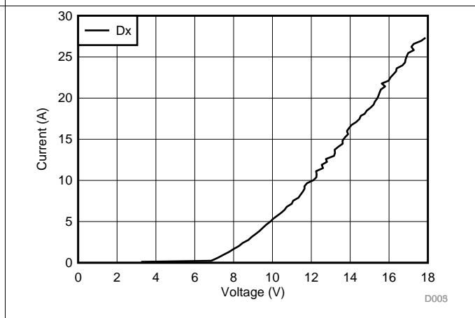
Figure 28. Dx TLP Curve
