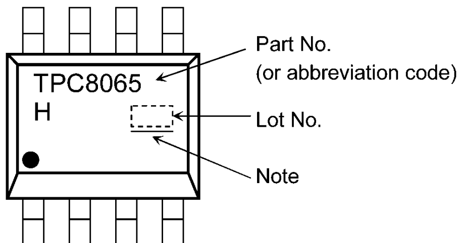
Fig. 7.1 Marking
