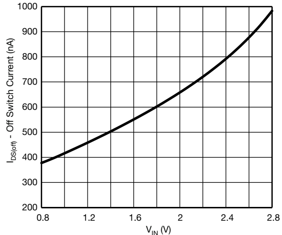
Fig. 8 - Off Switch Current vs. Input Voltage
