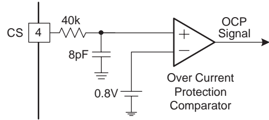
Figure 38. Over Current Protection Block
